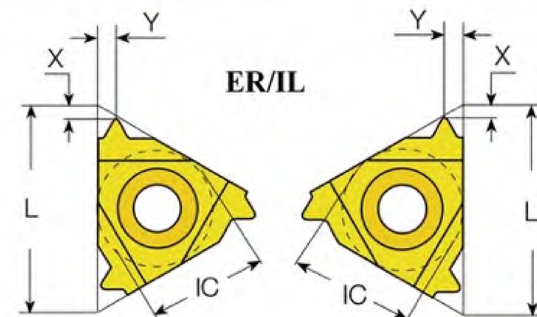
Metric Aerospace Full Profile Thread Insert
