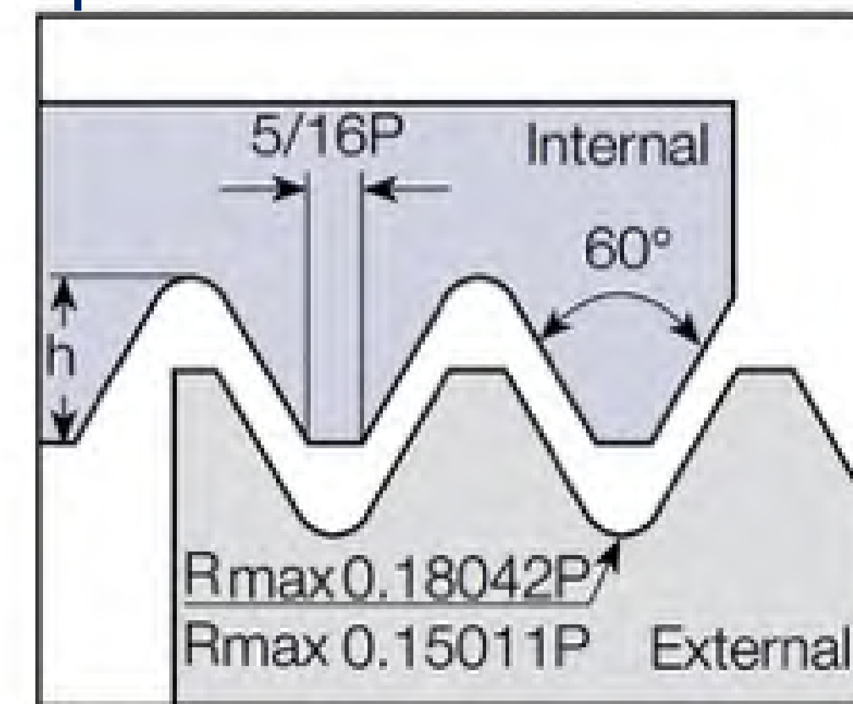
Metric Aerospace Full Profile Thread Insert
