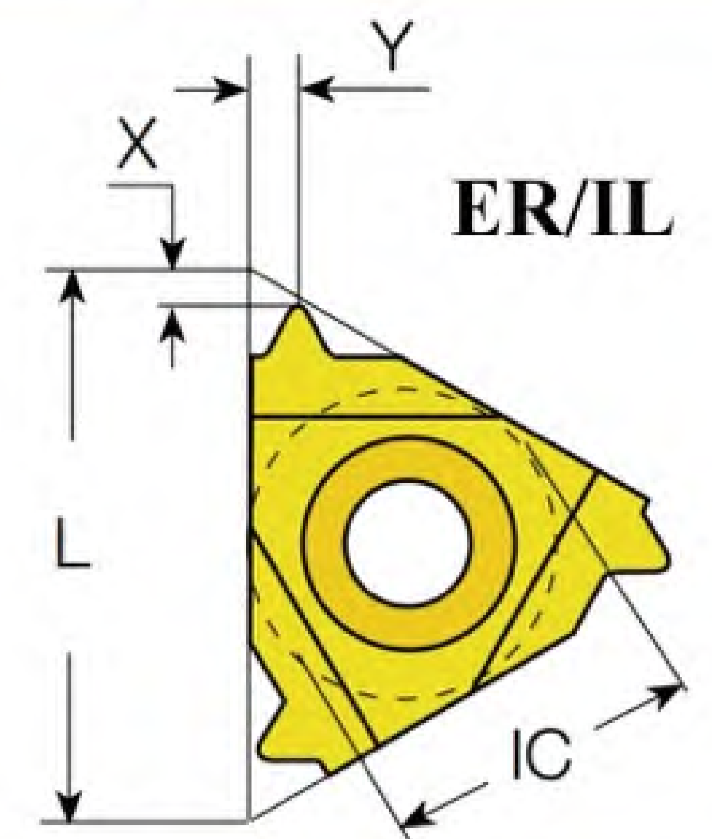
British Whitworth Full Profile Thread (BSW/BSF/BSP) 55°
