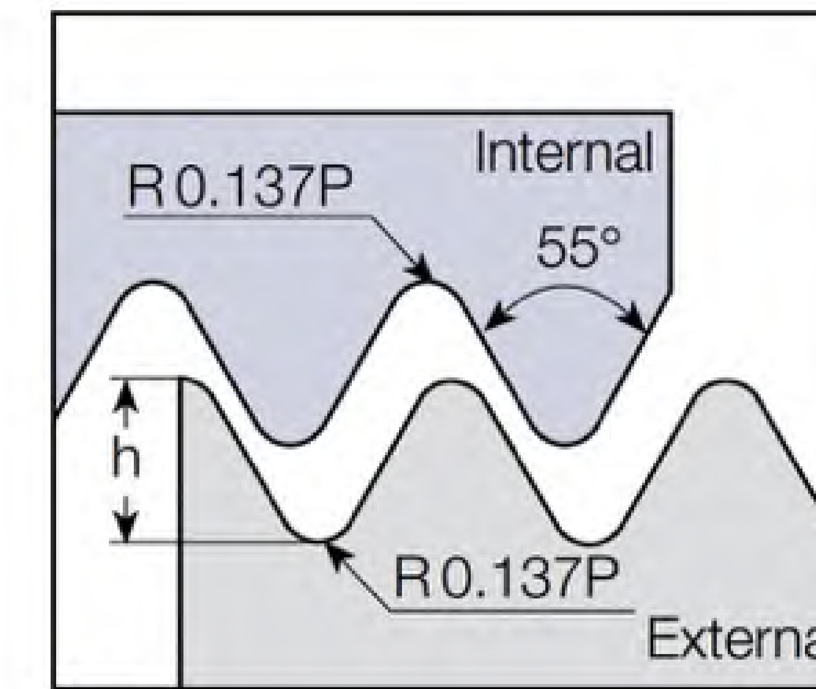
British Whitworth Full Profile Thread (BSW/BSF/BSP) 55°
